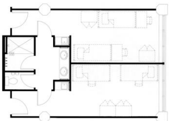
Type C – Double unit with one bathroom
